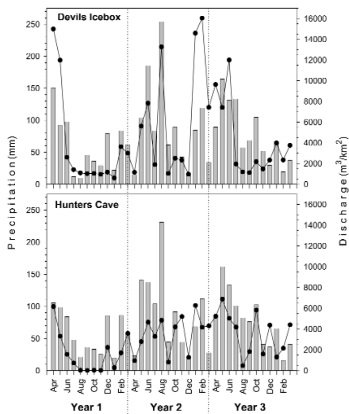
Figure 6. Monthly precipitation (bar graphs) within both recharge areas and monthly discharge (line graphs) for each cave stream at their resurgences.
